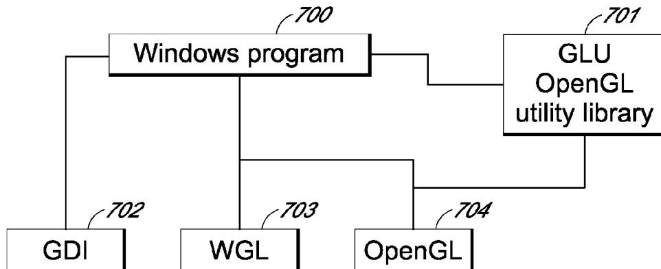
Algorithm
